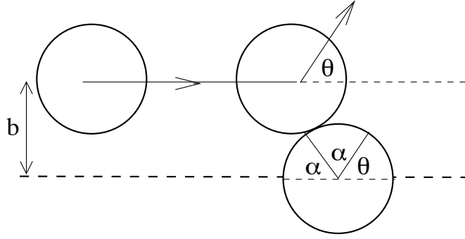
Figure 6: Hard sphere scattering from a hard sphere
