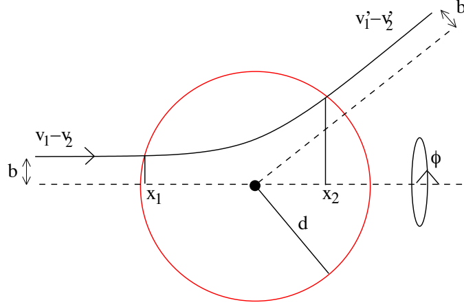
Figure 7: Two particle scattering.
