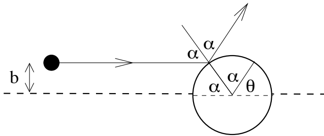
Figure 5: Particle scattering from a hard sphere
