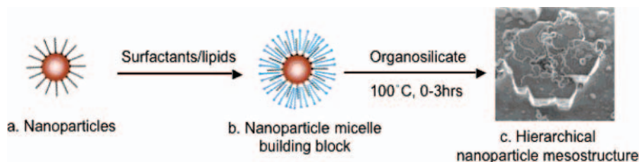
Scheme 1. Formation of the Water-Soluble Nanoparticle Micelle and Preparation of Hierarchical Nanoparticle Mesostructure Arrays through Hydrothermal Self-Assembly of Water-Soluble Nanoparticle Micelle Building Blocks with Organosilicate a
