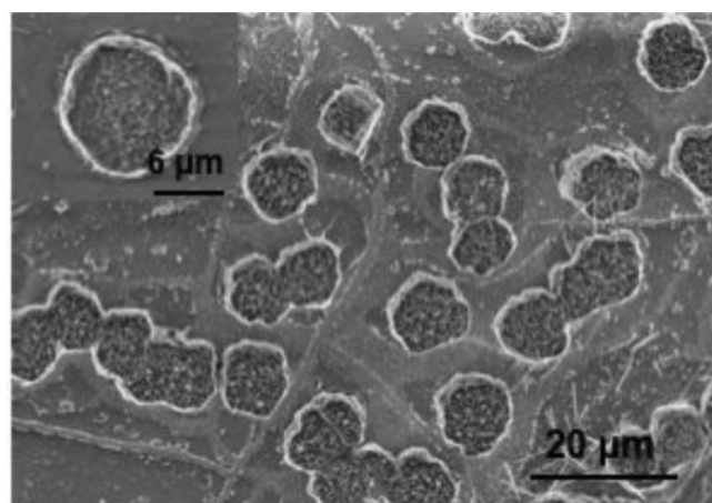
Figure 4. Representative SEM micrograph of hierarchical nanoparticle mesostructure arrays grown on a freshly peeled mica surface using BTEE as the precursor under basic conditions at 100 °C for 60 min. Inset: a magnified SEM image showing an individual mesostructure crystal.
