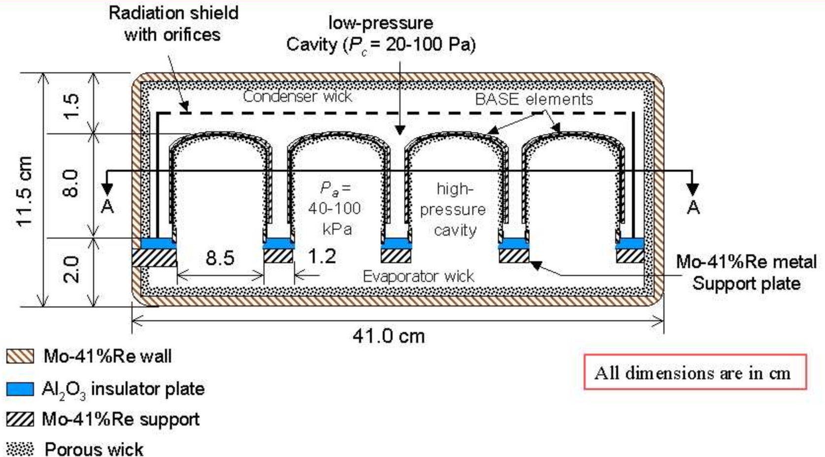
Elevation cross-sectional view B - B
