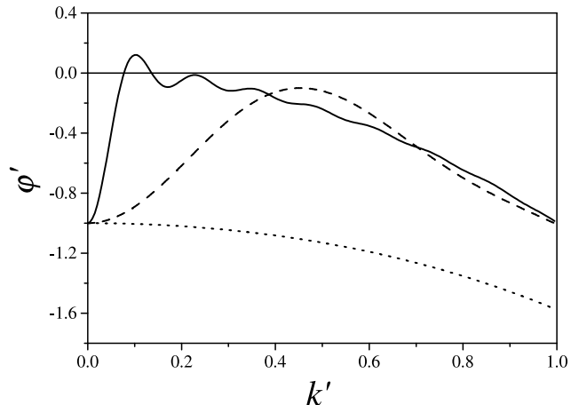
FIG. 2: The dispersion relation (15) between the dimensionless growth exponent \varphi' and wavenumber k' plotted for the intermediate influence function. Values of \eta are as in Fig. 1: 50 (solid line), 10 (dashed line), and 2 (dotted line). Patterns appear for those values of k' for which \varphi' is positive.
