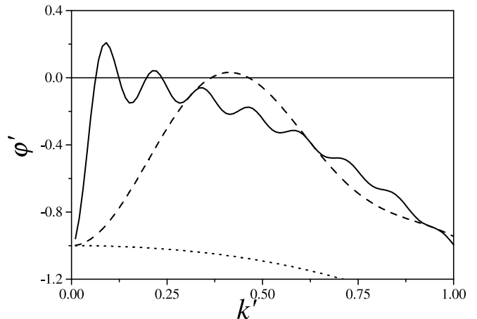
FIG. 1: The dispersion relation (9) between the dimensionless growth exponent \varphi' and wavenumber k' plotted for different values of the ratio \eta of the influence function range to the diffusion length (see text). Values of \eta are 50 (solid line), 10 (dashed line), and 2 (dotted line). Patterns appear for those values of k' for which \varphi is positive.
