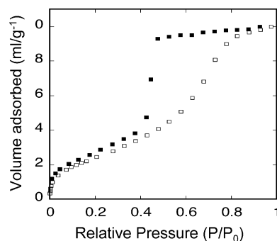
Figure 5. Nitrogen sorption isotherms of 3D nanoporous carbon films prepared by using turanose (7.1 wt%) and 0.1 gwt% PS-P4VP (polymer source, M_n^{PS} = 12\,000 g mol -1 , M_n^{PS} = 11\,800 g mol -1 with molecular size distribution of 1.04). The measurement was conducted at 77 k using surface acoustic wave techniques. The film was applied to \sim 1 cm 2 area of a piezoelectric ST-cut quartz substrate with interdigitated gold transducers designed to operate at \sim 97 MHz. Mass change was monitored ( \sim 80 pg cm -2 ) as a functional of relative pressure using a surface acoustic wave technique.
