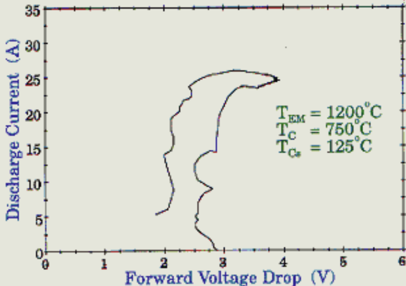
Typical I(V) Characteristic
