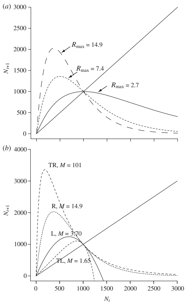
Figure 1. Plots of N_{t+1} versus N_t , illustrating the May threshold. (a) The May threshold is the value of R_{\max} at the transition to unstable dynamics (see electronic supplementary material, appendix SA for details). (b) The May threshold ( M ) for several well-known one- and two-parameter models of density-dependent population growth, evaluated approximately at the point where chaotic behaviour begins (as observed in simulations using these equations, see electronic supplementary material, appendix SA for details); R = Ricker [1,21]; L = logistic [1]; TR = \theta -Ricker [4], r = 4.62 , \theta = 0.585 ; TL = \theta -logistic [4,22], r = 0.50 , \theta = 5.50 . The two-parameter examples in the figure represent pairs of parameters that result in marked asymmetry of the density-dependence curve, chosen to illustrate the wide range in variation in M that is possible even with these simple models.
