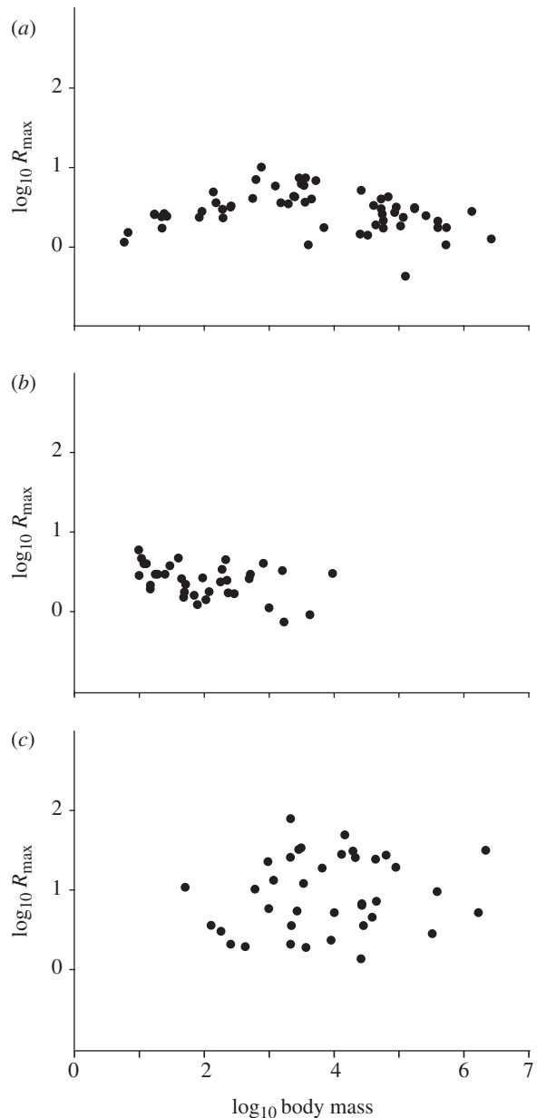
Figure 2. Maximum generational growth rate ( R_{\max} ) versus body mass ( B , in g), for groups of vertebrates spanning a large range of sizes and for which species R_{\max} values are available from the literature. Both variables are \log_{10} -transformed, since our prediction is that the ordinary least-squares slope of such a relationship will not differ from 0. For three independent tests, a Bonferroni corrected p -value of \leq 0.017 is required to indicate a significant departure from 0 at the 0.05 level [23]. (a) Mammals, \log R_{\max} = 0.55 - 0.03(\log B) , p = 0.17 , n = 58 ; R_{\max} estimated as the product of annual birthrate and average female lifespan; adapted from Purvis & Harvey [24]. (b) Birds, \log R_{\max} = 0.89 - 0.10(\log B) , p = 0.023 , n = 36 ; R_{\max} estimated as average lifetime production of female fledglings; see electronic supplementary material, appendix SC for data and sources. (c) Fishes, \log R_{\max} = 0.68 + 0.068(\log B) , p = 0.34 , n = 38 ; estimates of R_{\max} based on empirical spawner-recruitment curves (number of reproducing females per generation; [25]); maximum reproductive rate is the slope at the origin for the fit of a Ricker-like model to the data.
