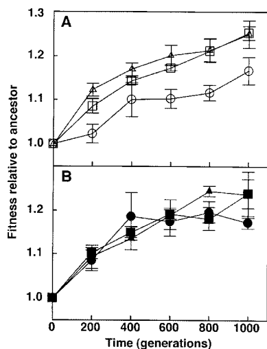
Fig. 1. Fitness trajectories of wild-type and mutator populations, founded by the nonadapted strain, during experimental evolution. Points indicate the average fitness of four populations in each treatment relative to the corresponding ancestor; error bars show standard errors. Circles are wild type, squares mutY , triangles mutS . (A) Small effective population size ( = 6.6 \times 10^5 ). (B) Large effective population size ( = 3.3 \times 10^7 ).
