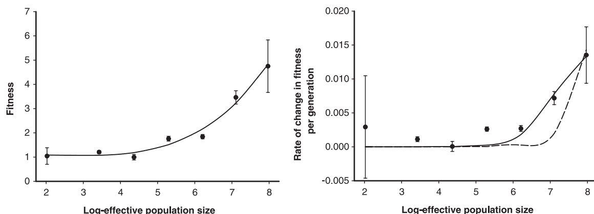
Fig. 1 (left). Influence of effective population size on the magnitude of the fixed fitness effect. Error bars represent standard errors ( n = 5 ). The solid line represents the fit to the theoretical model described in brief in (13) and in more depth in (4). Fig. 2 (right). Influence of effective population size on the rate of evolution. Error bars represent standard errors ( n = 5 ). Because the rate of adaptation in an asexual population of size zero must be null, the y intercept has been fixed at zero. The dashed line represents the fit of the experimental data to a linear model. The solid line represents the fit to a hyperbolic model [ R^2 = 0.8710 ,
