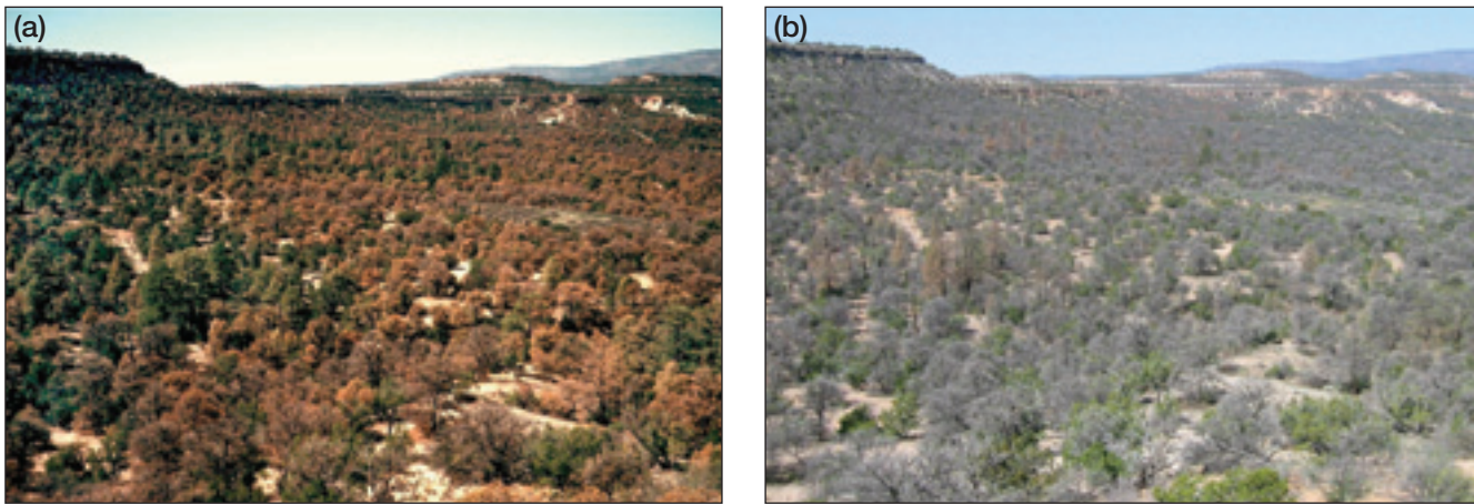
Figure 2. Landscape transformation associated with a die-off of piñon pine trees ( Pinus edulis ) triggered by a global change-type drought. Piñon pine trees, evergreen when alive, (a) exhibiting reddish-brown foliage indicating mortality (October 2002). (b) After they have lost their needles, exposed gray trunks of standing dead tree carcasses remain (May 2004). Almost all of the surviving green trees in (b) are junipers.
