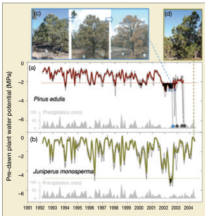
Figure 3. Pre-dawn plant water potential (more negative values indicate greater water stress) for (a) piñon ( Pinus edulis ; reddish-brown line) and (b) juniper ( Juniperus monosperma ; olive line). Thin, gray lines indicate individual trees, thick lines indicate species means of living trees, shaded gray indicates monthly precipitation. (c) Foliar progression from dark green to pale green to brown for an individual piñon (May to August to October 2002, corresponding with blue inset box and blue mortality point in [a]; other piñon mortality points in dark gray); (d) junipers survived. Straight lines (color coded by species) are set at zero assimilation points for both piñon and juniper; black shaded areas below these lines highlight periods of accumulated water stress.
