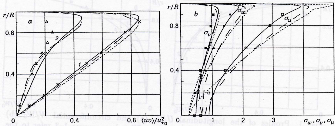
Fig. 3. Components of the turbulent stress tensor: (a) shear stress \langle uv \rangle / u_{*0}^2 for SP = 0 and 0.6; (b) normal stress for SP = 0; the experimental points \square , \bullet , and \blacktriangle correspond to \sigma_u = \langle u^2 \rangle / u_{*0}^2 , \sigma_v = \langle v^2 \rangle / u_{*0}^2 , and \sigma_w = \langle w^2 \rangle / u_{*0}^2 ; see also the legend in Figs. 1 and 2.
