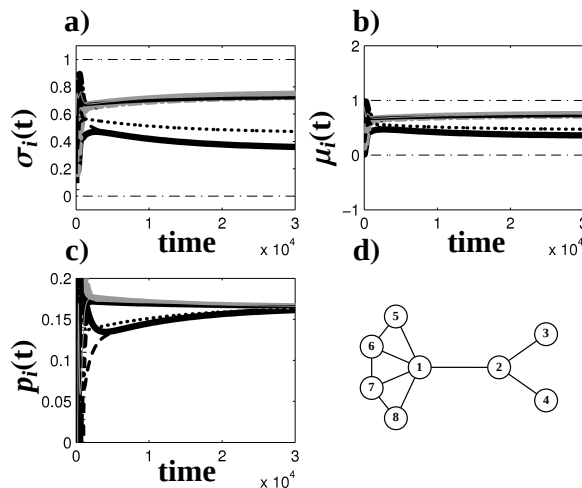
FIG. 2: We consider an 8-node network, shown in plot d. The benefit of cooperation is set to b = 1.1 ( c = 1 ). Plot a shows the time evolution of \sigma_i(t) , i = 1, \dots, 8 , with all the strategies \sigma_i(t) converging on a fully mixed state, corresponding to \bar{v}_0 . Plot b shows the evolution of \mu_i(t) , i = 1, \dots, 8 . Plot c shows the evolution of p_i(t) , i = 1, \dots, 8 , with all the payoffs converging after a transient to 0.165. The initial conditions for \mu 's and \sigma 's are randomly chosen from a uniform distribution in the interval (0, 1) , \alpha = 5 \times 10^{-2} , \beta = 10^{-3} , \gamma = 1 .
