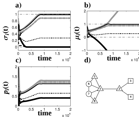
FIG. 3: We repeat the simulation in Fig. 2, but now the benefit of cooperation b = 1.5 . With this choice of the parameters, the fully mixed state is unstable. Plot a shows the time evolution of \sigma_i(t) , i = 1, \dots, 8 . Nodes 3 and 4 (shown as squares in the graph) converge on the defector state (0); nodes 6 and 7 (shown as circles in the graph) converge on the cooperator state (1); the remaining four nodes (shown as triangles) converge on a mixed strategy. Plot b shows the evolution of \mu_i(t) , i = 1, \dots, 8 . Plot c shows the evolution of the payoffs p_i(t) , i = 1, \dots, 8 , which converge on different final values: p_1 = 1.13, p_2 = 0.652, p_3 = 0.411, p_4 = 0.411, p_5 = 1.21, p_6 = 1.29, p_7 = 1.29, p_8 = 1.21 . The initial conditions for \mu 's and \sigma 's are randomly chosen from a uniform distribution in the interval (0, 1) , \alpha = 5 \times 10^{-2} , \beta = 10^{-3} , \gamma = 1 .
