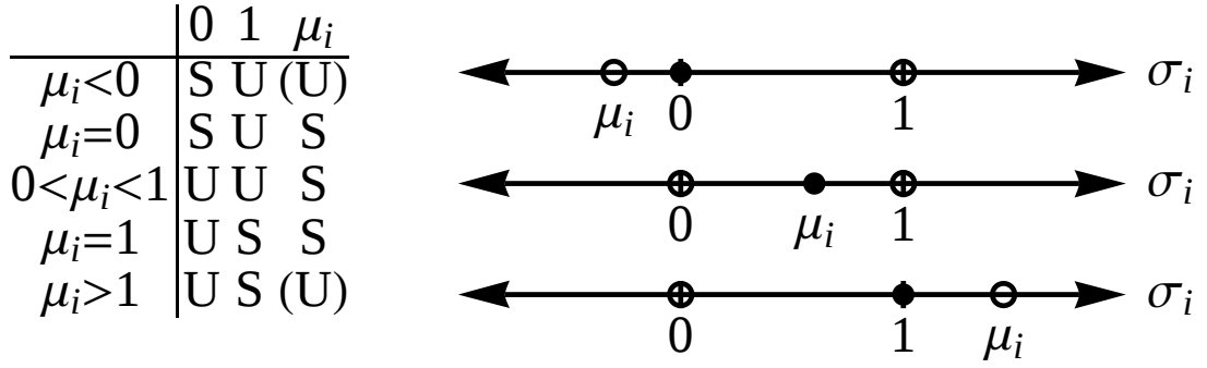
FIG. 1: The table (on the left) shows the stability (S) or instability (U) of each of the fixed points \{0, 1, \mu_i\} for any occurrence of \mu_i . Note that the stability of the fixed points \sigma_i = \mu_i for \mu_i > 1 and for \mu_i < 0 is in brackets as these equilibria are never observed if \sigma_i(0) \in (0, 1) . On the right, we have a graphical representation of the stability of the fixed points of Eq. (6a) for different values of \mu_i , where open circles represent unstable fixed points and filled circles represent stable ones. From top to bottom, we show the cases of \mu_i < 0 , 0 < \mu_i < 1 , and \mu_i > 1 .
