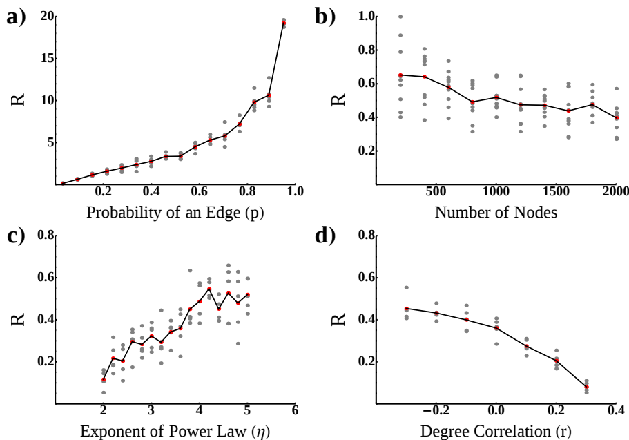
FIG. 5: Plot (a) shows the range of stability R (shown in Fig. 4(a)) for random Erdős-Rényi graphs of 200 nodes versus the probability of an edge parameter p , for 5 different cases (grey points) for each p , with the average R connected by line segments. Plot (b) shows the range of stability R for random Erdős-Rényi graphs of dimension N and average degree fixed and equal 20, for 10 different cases (grey points) for each N , with the average R connected by line segments. Plot (c) shows the range of stability R for scale free networks of 200 nodes versus the exponent of the degree distribution, \eta , where the average degree is kept fixed at 20. Plot (d) shows the range of stability R for scale free networks of 200 nodes, \eta = 3.5 , average degree equal 20, versus the degree correlation coefficient r .
