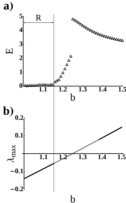
FIG. 4: Plot (a) shows the result of evolving the network in Fig. 2d for a long time from random initial conditions in the range (0, 1) . We plot the deviation E of the final state from the state associated with the eigenvector \bar{v}_0 as a function of the game parameter b for c = 1 . The label R represents the range of stability. Plot (b) shows the largest nonzero eigenvalue of the matrix B versus b . The grey section of the curve represents the range over which the entries of the eigenvector \bar{v}_0 are not all of the same sign.
