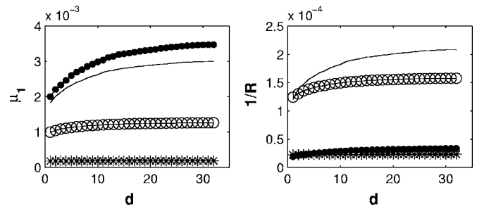
FIG. 12. A square lattice of 32 \times 32 nodes is considered. Assuming that two of its nodes have been chosen to be controlled, the controllability indices \mu_1 and 1/R are plotted vs their distance d . Different lines indicate different control gains \kappa : \kappa=10^{-1} (asterisks), \kappa=10^0 (circles), \kappa=10^1 (no marker), and \kappa=10^2 (dots).
